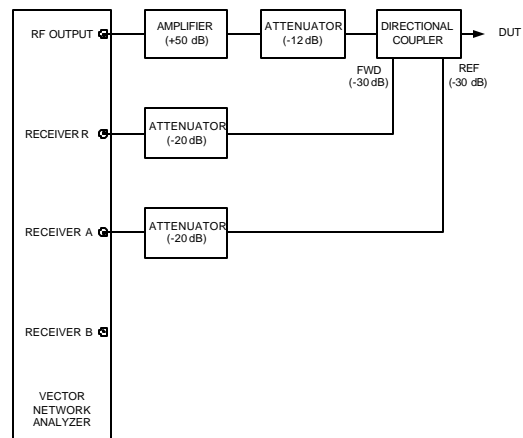
IMPEDANCE MEASUREMENT SYSTEM
